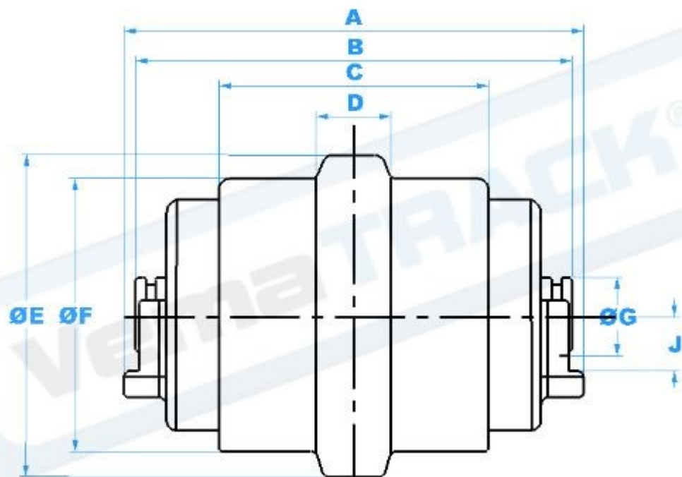
6 Track Roller
