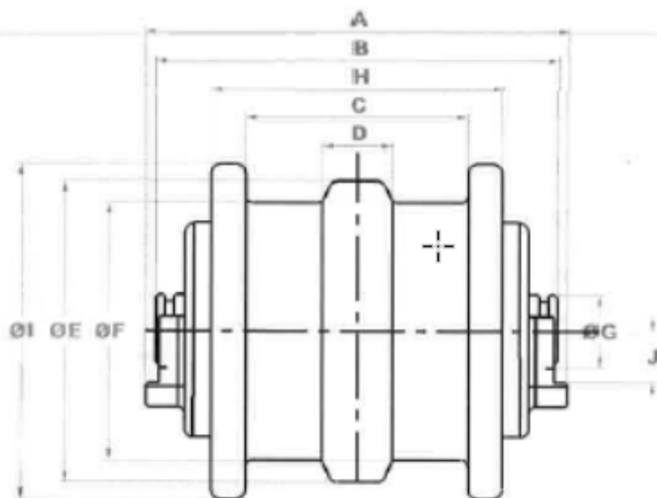
G12 Track Roller
